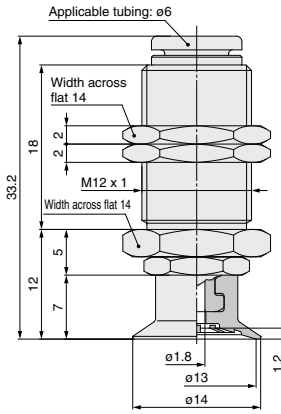
ZP3-T13UM□-A12-06
