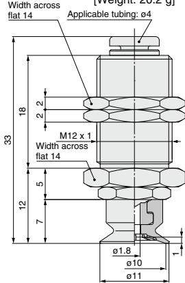
ZP3-T10UM□-A12-04
