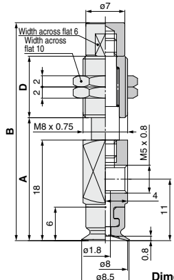
ZP3-Y08UM□J■-B5
