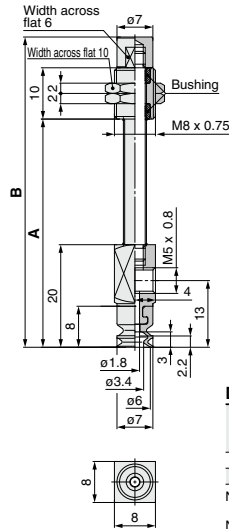
ZP3-Y06B□JB■-B5
