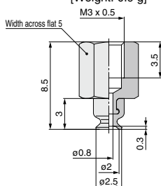
ZP3-T02U□-A6-B3
