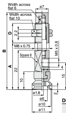
ZP3-Y10B□J■-B5
