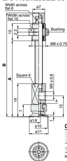
ZP3-Y10UM□JB■■-B5
