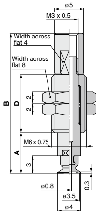
ZP3-T035U□J■-B3
