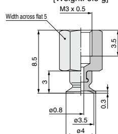
ZP3-T035U□-A6-B3
