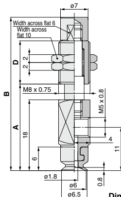
ZP3-Y06UM□J■-B5
