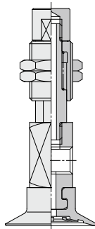
ZP3-Y16UM□K■-B5
