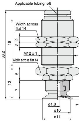
ZP3-T10UM□-A12-06
