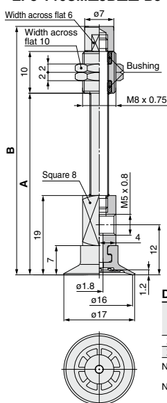
ZP3-Y16UM□JB■■-B5
