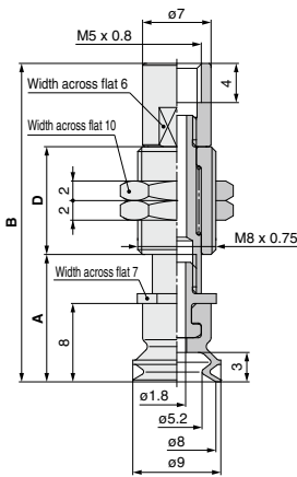
ZP3-T08B□J■-B5
