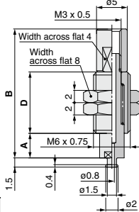
ZP3B-T1J■-B3
