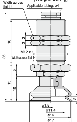
ZP3-T16B□-A12-04
