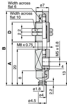
ZP3-Y04B□J■-B5
