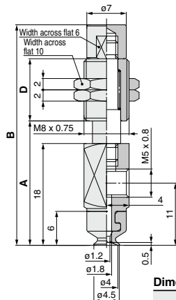
ZP3-Y04UM□J■-B5
