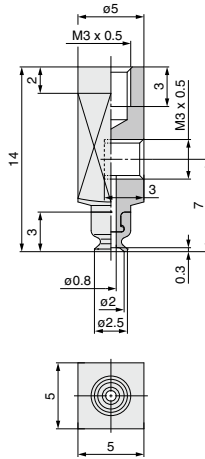
ZP3-Y02U□-B3-B3
