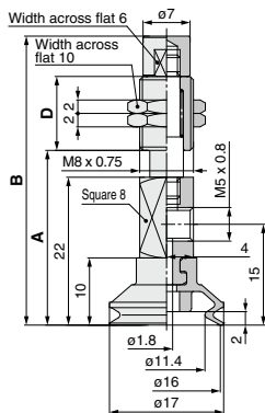
ZP3-Y16B□J■-B5
