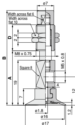
ZP3-Y16UM□J■-B5
