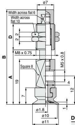
ZP3-Y10UM□J■-B5
