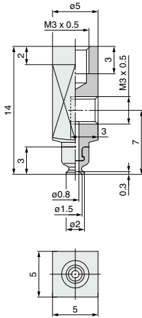
ZP3-Y015U□-B3-B3
