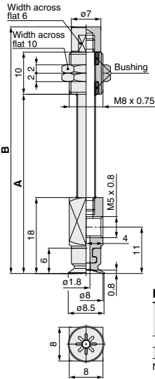
ZP3-Y08UM□JB■-B5
