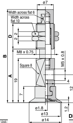
ZP3-Y13UM□J■-B5
