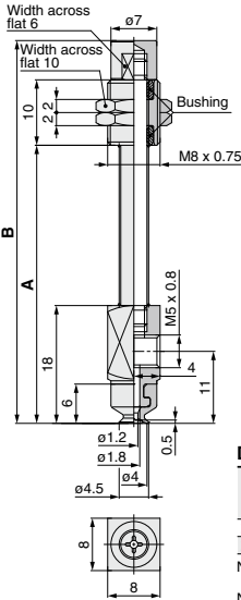
ZP3-Y04UM□JB■-B5
