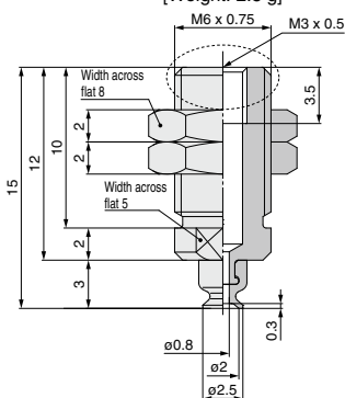
ZP3-T02U□-A6-B3
