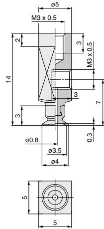
ZP3-Y035U□-B3-B3
