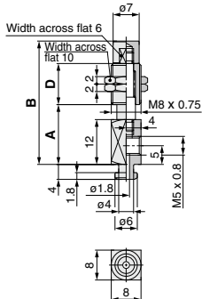
ZP3B-Y2BJB■■-B5
