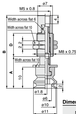
ZP3-T10B□J■-B5
