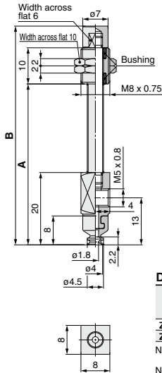
ZP3-Y04B□JB■-B5
