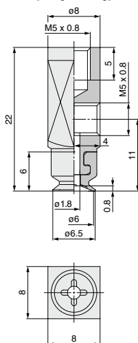
ZP3-Y06UM□-B5-B5
