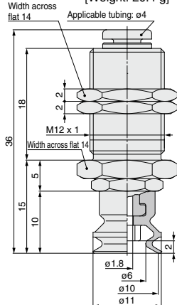
ZP3-T10B□-A12-04
