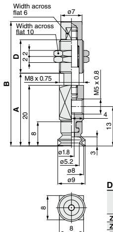
ZP3-Y08B□J■-B5
