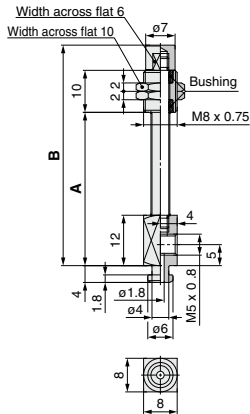
ZP3B-Y2BJB■■-B5
