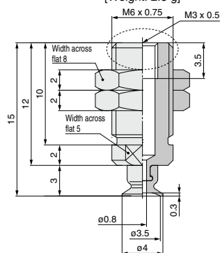
ZP3-T035U□-A6-B3
